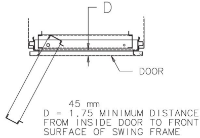
120° Mounting Position
